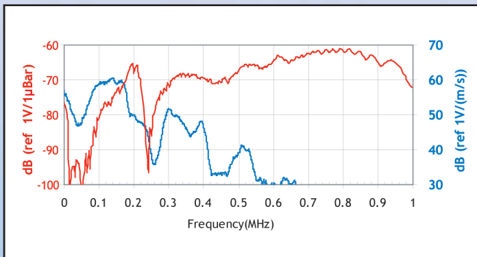
Frequency response of the R80α. Calibration based on ASTM E1106; Calibration based on ASTM E976.
